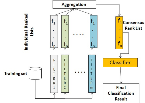
Fig. 2. Feature Selector Based Aggregation
